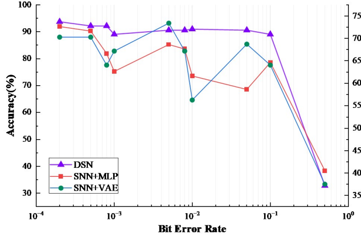
Fig. 7. Comparison of the accuracy of DSN and SNN with other classifiers under bit error conditions.
